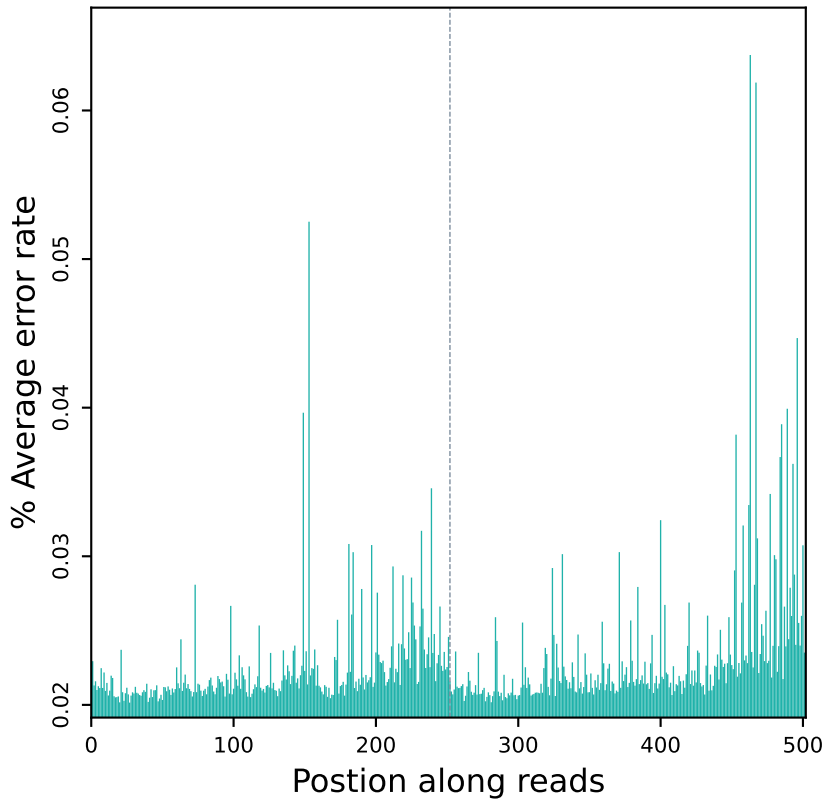
Error rate distribution along reads (R10822)
